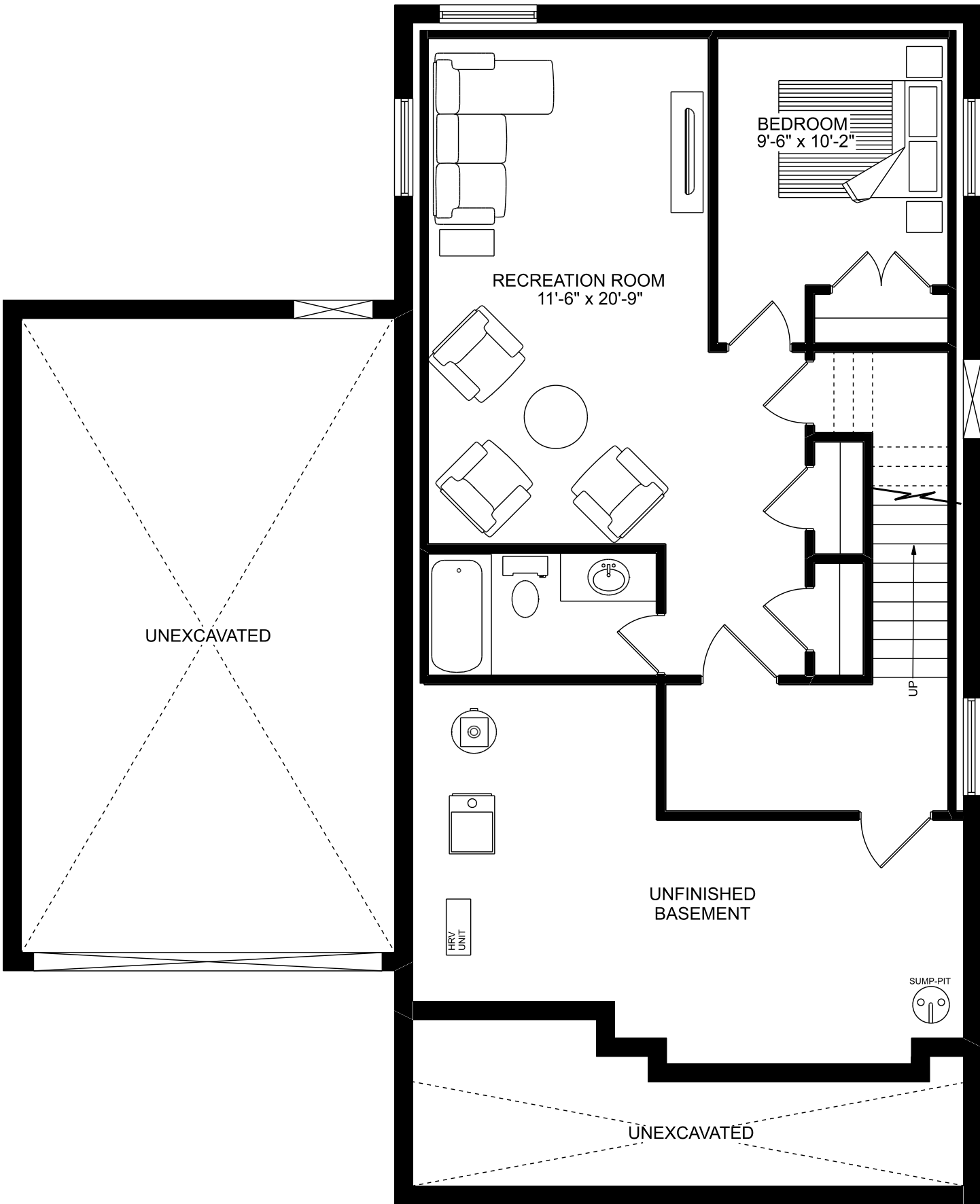
FINISHED BASEMENT PLAN 550 SQ.FT.
