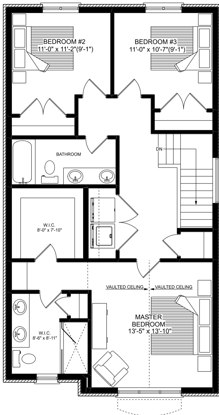
UPPER FLOOR PLAN 1025 SQ.FT.
