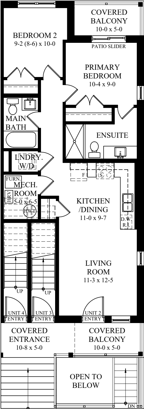
MAIN LEVEL FLOOR PLAN END UNIT 2 - 788 sq.ft. END UNIT 3 (FRONT) - 59 sq.ft. END UNIT 4 (REAR) - 60 sq.ft.
