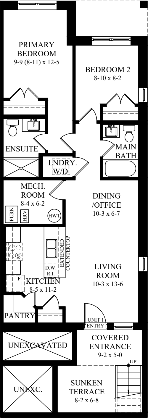
TERRACE LEVEL FLOOR PLAN END UNIT 1 - 907 sq.ft.
